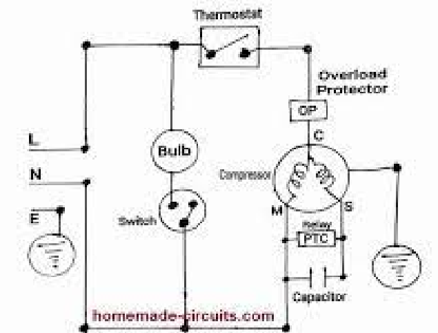
Circuit Diagram of today's Single Door Refrigerator
